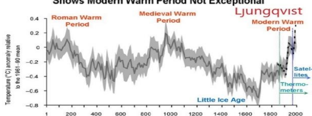
Temperature Reconstruction* for N. Hemisphere, 1 - 2000 AD Shows Modern Warm Period Not Exceptional
